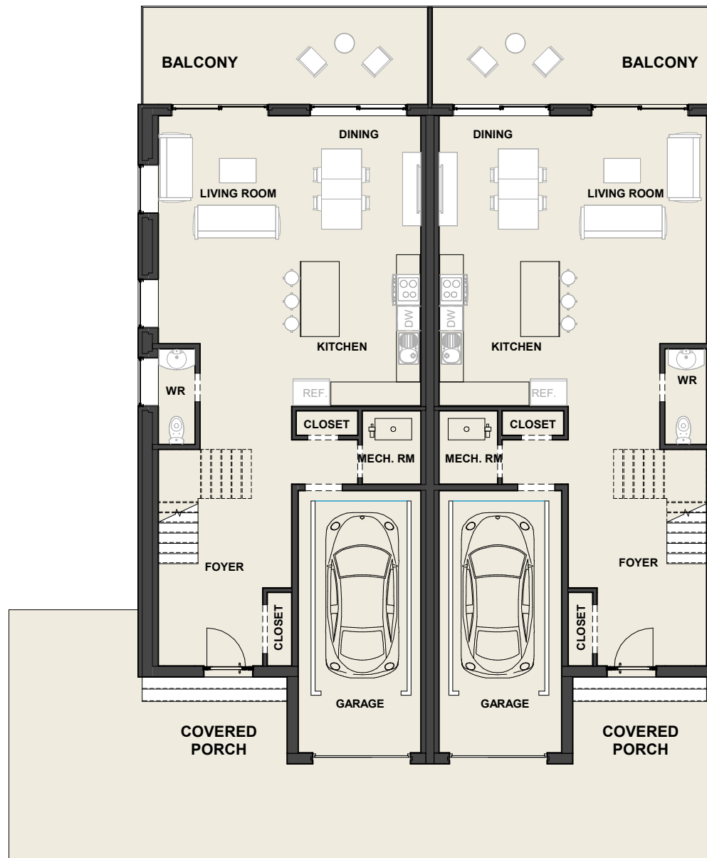
FIRST FLOOR FURNITURE LAYOUT
